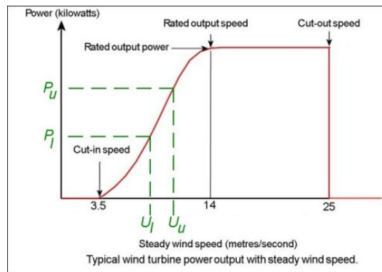
Figure 1: Wind turbine power profile 2
